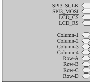
U_User Interface User Interface.SchDoc
